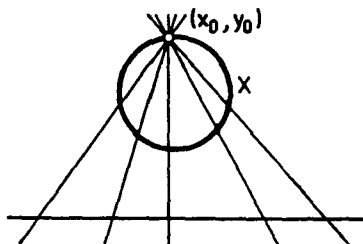
Figure 4. Projection of a Conic
