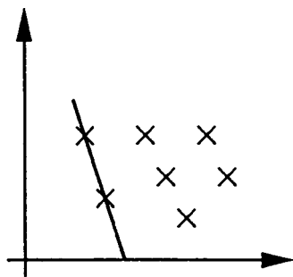
Figure 11. The Newton Polygon
