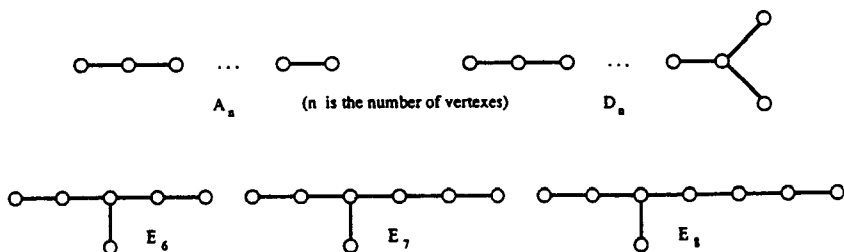
Figure 20. The Dynkin Diagrams A_n , D_n , E_6 , E_7 and E_8
