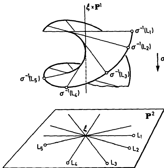
Figure 10. The Blowup \sigma: \Pi \rightarrow \mathbb{P}^2
