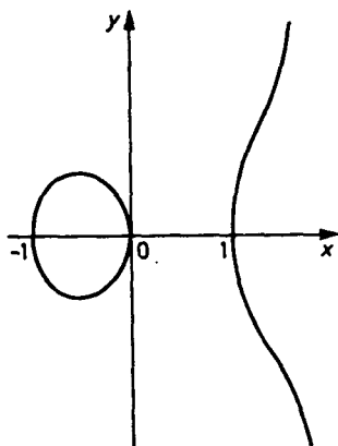
Figure 8. y^2 = x^3 - x over \mathbb{R}
