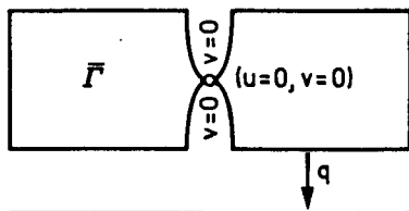
Figure 15. The Map f(x, y) = xy
