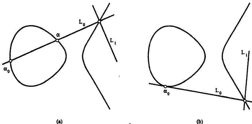
Figure 12. Constructing Functions on a Plane Cubic
