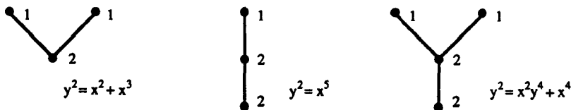
Figure 19. Resolutions of Some Curve Singularities
