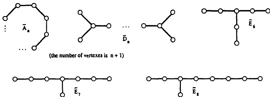
Figure 21. The Extended Dynkin Diagrams \bar{A}_n , \bar{D}_n , \bar{E}_6 , \bar{E}_7 and \bar{E}_8
