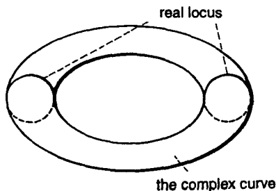
Figure 9. y^2 = x^3 - x over \mathbb{C}
