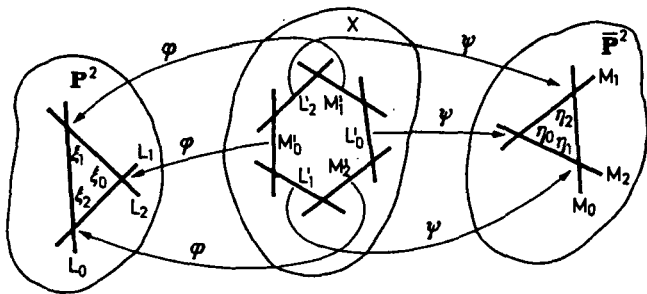
Figure 18. The Standard Quadratic Transformation
