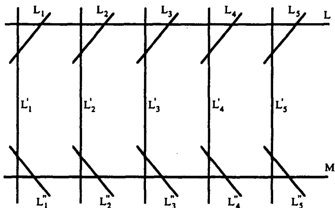
Figure 17. Lines on the Cubic Surface
