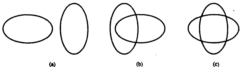
Figure 1. Intersections of Conics
