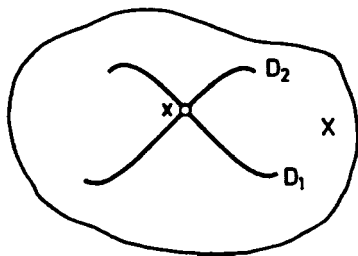
Figure 7. Transversal Curves on a Surface
