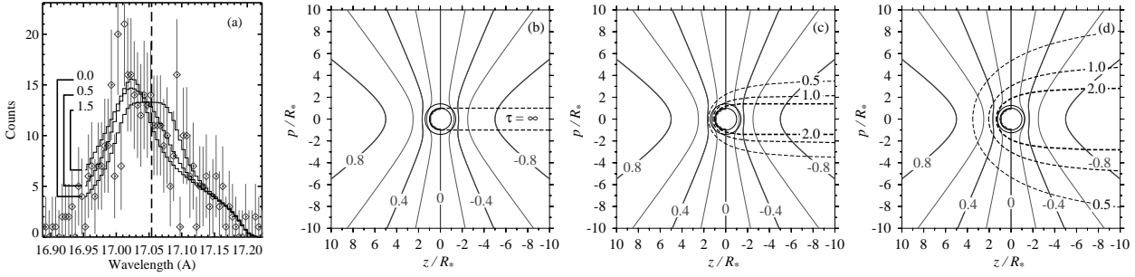
FIG. 2.— Models at extremes of the confidence region. Shown are the Chandra MEG spectrum of the 17.054 Å line of Fe XVII (in gray), and (in black) the best-fit model ( \tau_* = 0.5 ), the fit with \tau_* held at its 95.4% confidence upper limit ( \tau_* = 1.5 ) and the fit with \tau_* held at its 95.4% confidence lower limit ( \tau_* = 0.0 ). The contour plots are the same style as in Figure 1 and correspond to (b) the \tau_* = 0.0 model, (c) the best-fit model, and (d) the \tau_* = 1.5 model.
